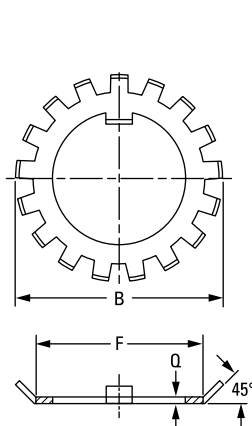
Fig. 50. Lockwashers.
